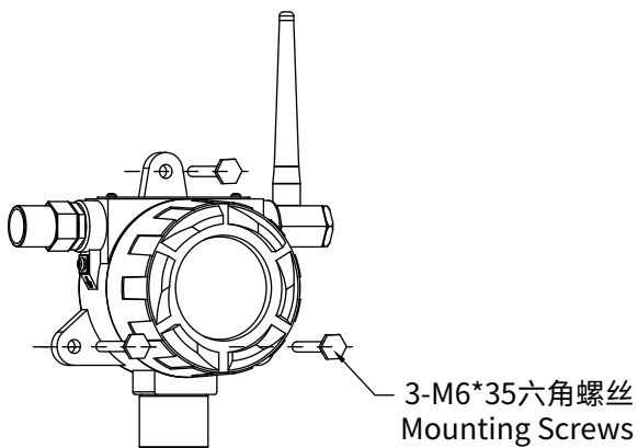
壁挂式安装 Wall-mounted Installation
