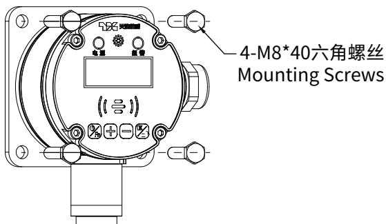
壁挂式安装 Wall-mounted Installation
