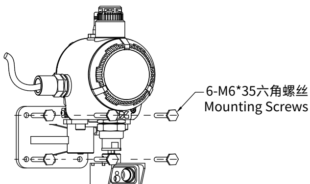
壁挂式安装 Wall-mounted Installation
