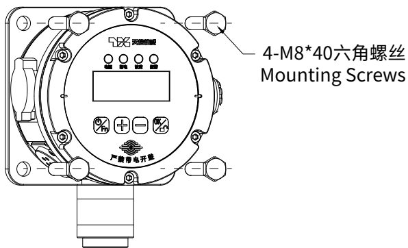
壁挂式安装 Wall-mounted Installation
