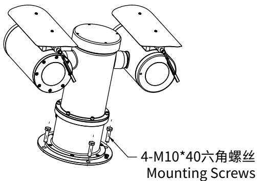
壁挂式安装 Wall-mounted Installation
