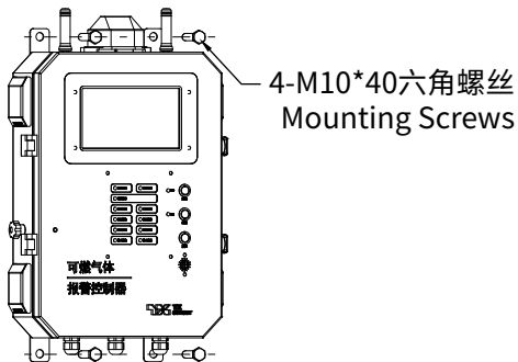
壁挂式安装 Wall-mounted Installation
